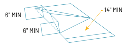
CRICKET FLASHING
