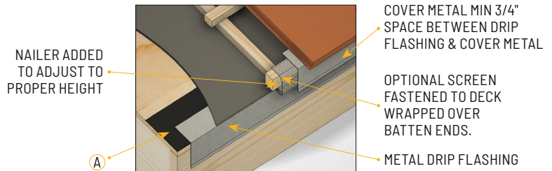
COUNTER BATTEN
