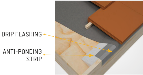
RAISED FASCIA
