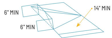
CRICKET FLASHING
