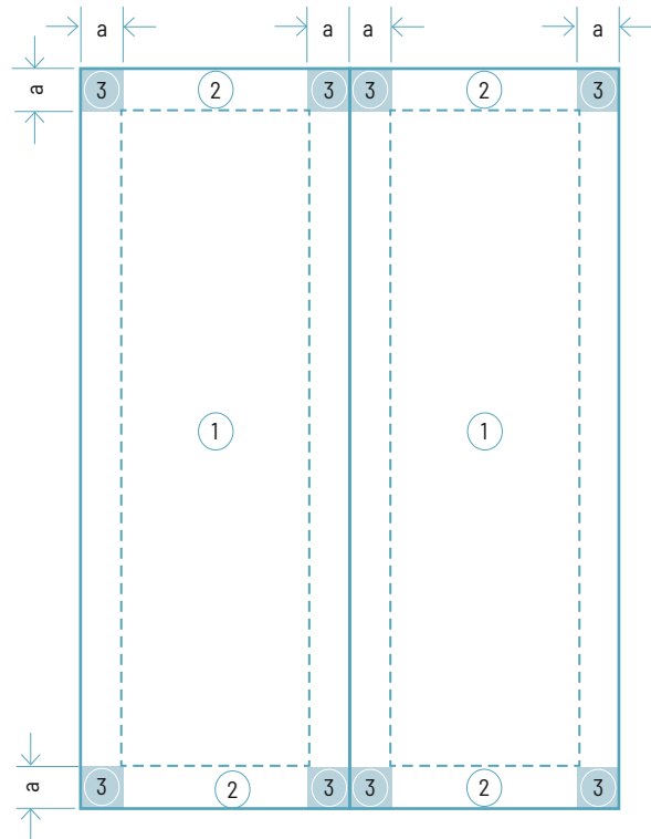
FIGURE 4.0 GABLE ROOF ZONE DESIGNATION
