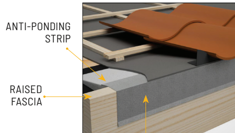
DRIP FLASHING
