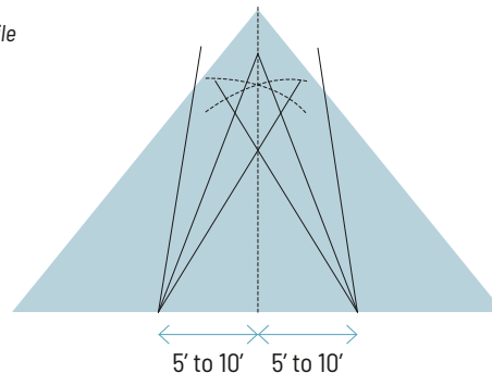
Drawing shown depicts the application of all tile profiles. Unless otherwise noted, it would apply to either concrete or clay tiles.
