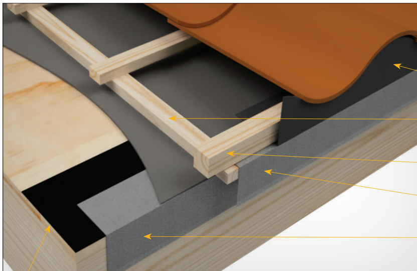
HIGH PROFILE TILE WITH BIRD STOP
